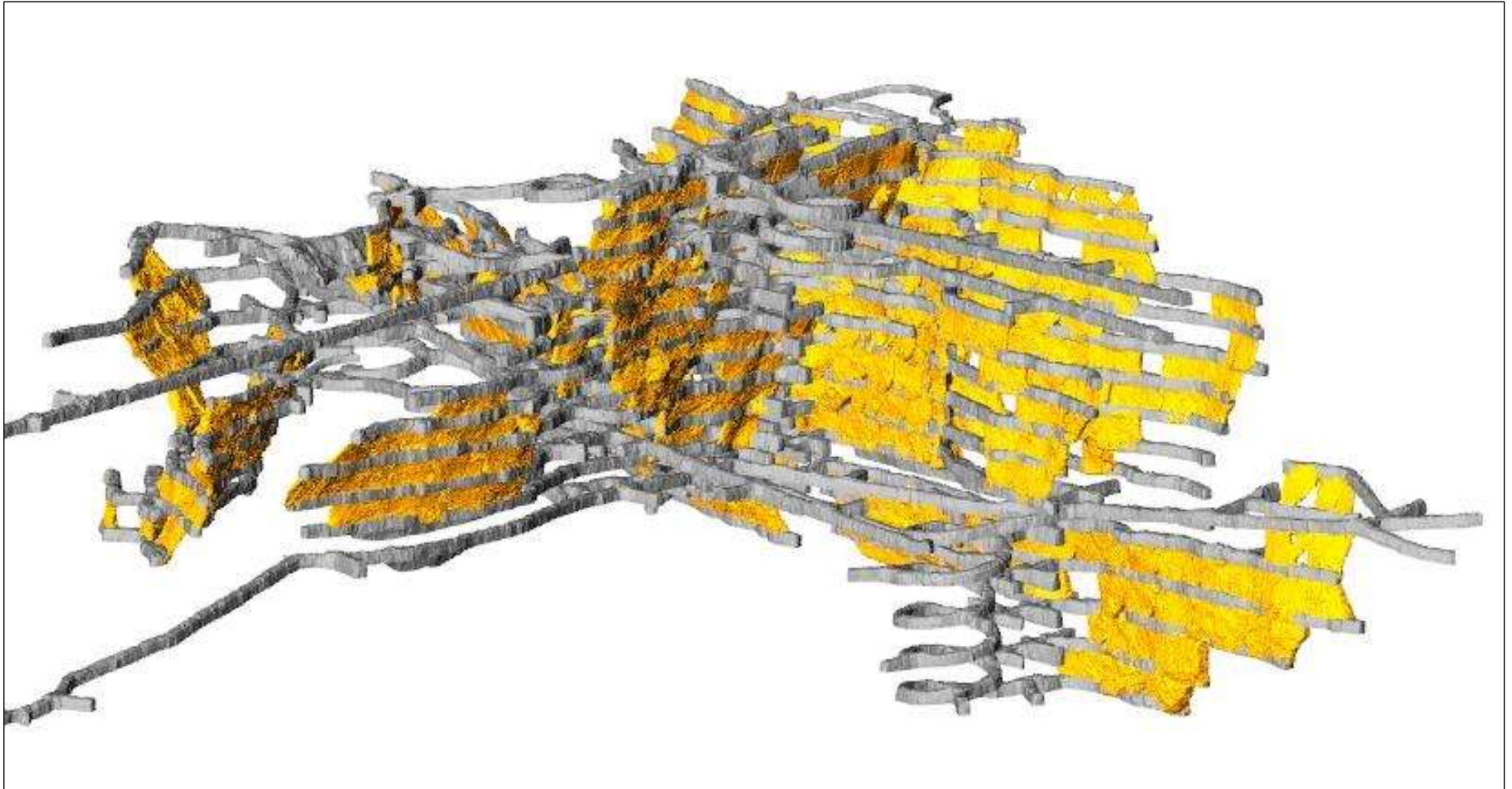
Figure 3: Oblique view of Correnso showing completed development (grey) and stopping activities (orange). View is looking northeast.
