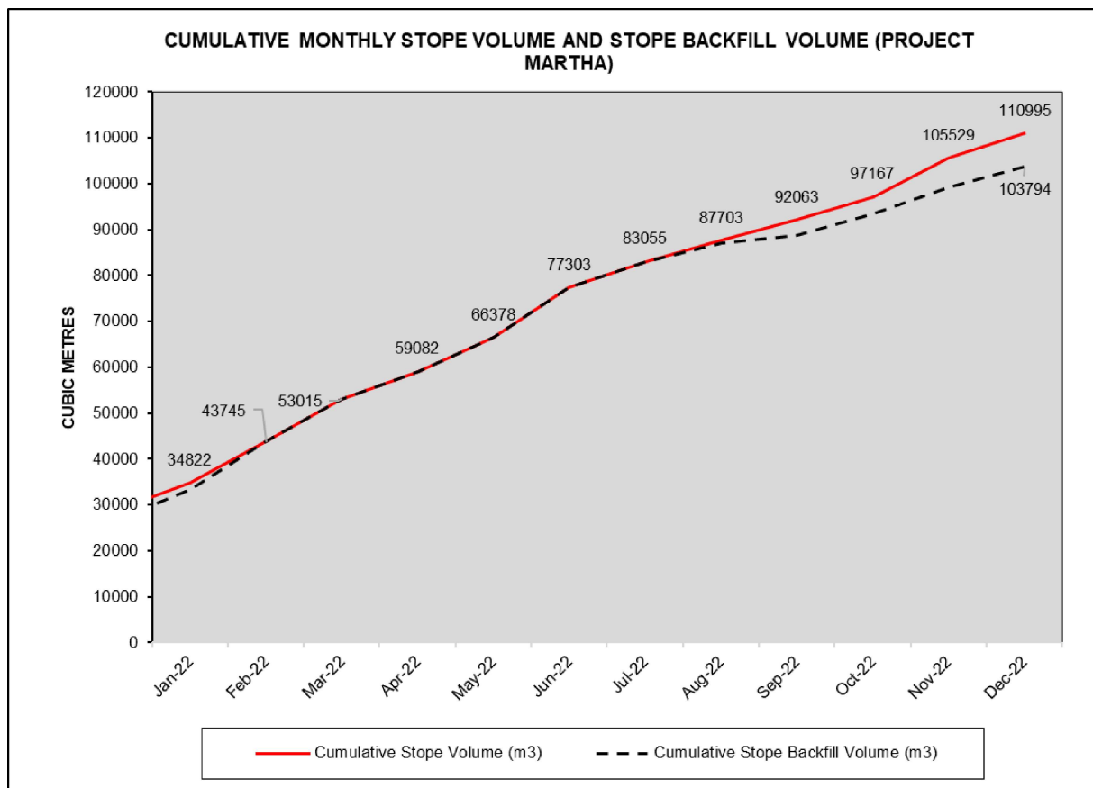
Figure 2: Martha Underground cumulative monthly stope voids and backfill volumes 2022
