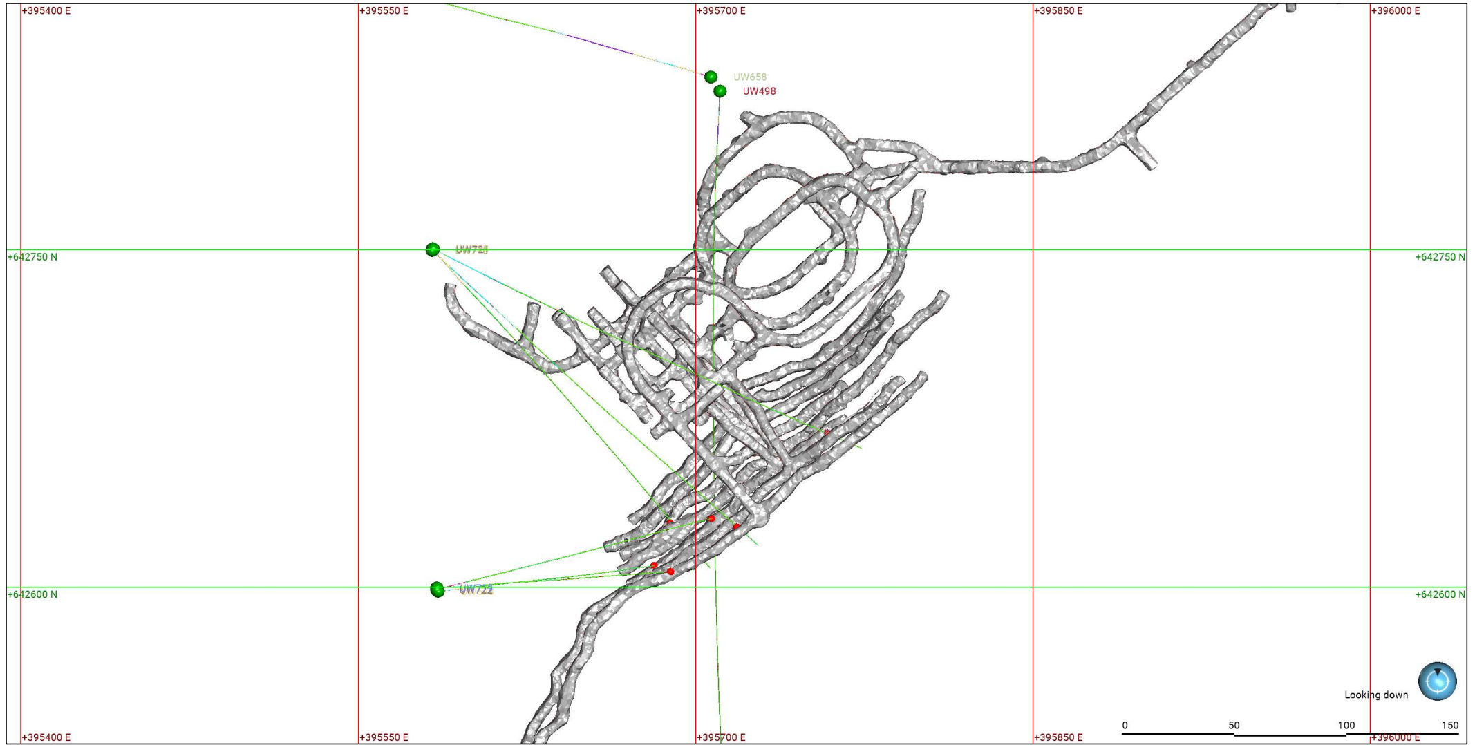
Figure 3: Surface holes intercepting underground workings, Rex
