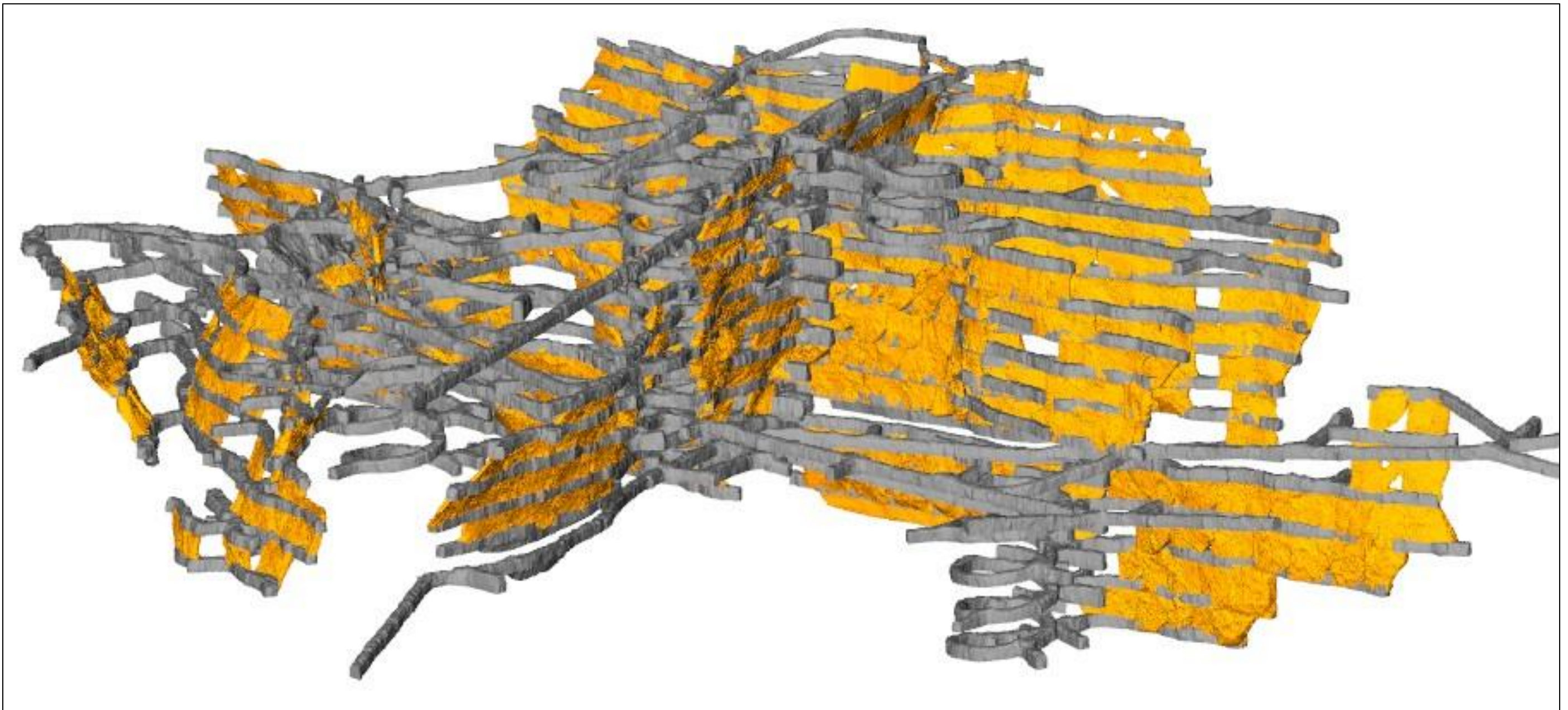
Figure 1: Oblique view of Correnso showing completed development (grey) and stoping (yellow) activities. View is looking northeast.
