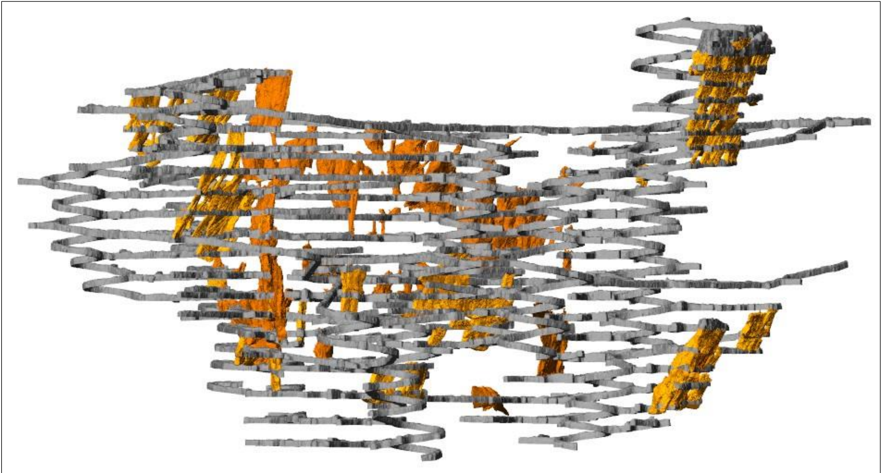
Figure 2: Oblique view of Martha Underground showing completed development (grey) and stoping (yellow) activities. View looking northeast.
