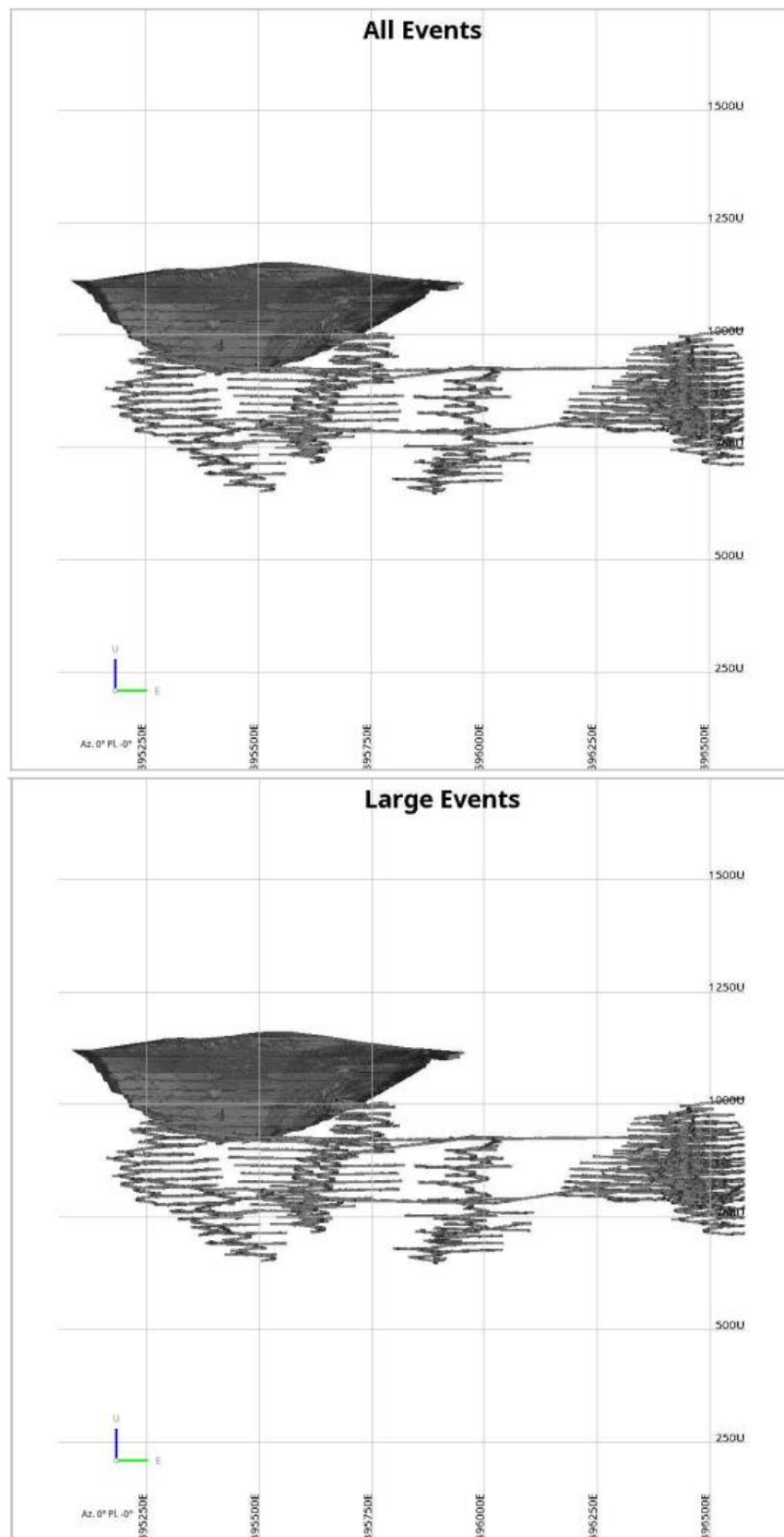
Figure 4: Section View showing location of triggered events & reportable large events. None > ML -0.5 during April 2025.
