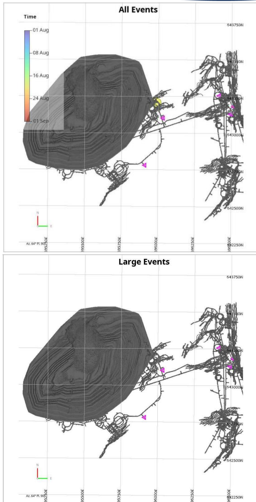
Figure 3: Plan View, Top: Normal (Location and Source) & m_L \geq -3.0 & number of accepted triggers \geq 3 , Bottom: Listing of events m > -0.5 during August 2025.
