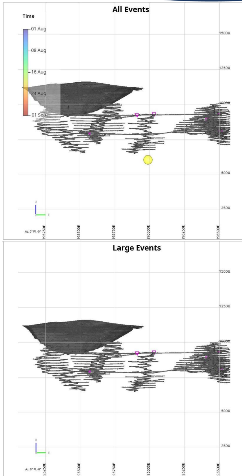
Figure 4: Looking North, Top: Normal (Location and Source) & mL \geq -3.0 & number of accepted triggers \geq 3 , Bottom: Listing of events m > -0.5 during August 2025.
