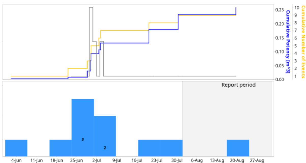
Figure 5: 3 Month Event History vs Cumulative Potency.
