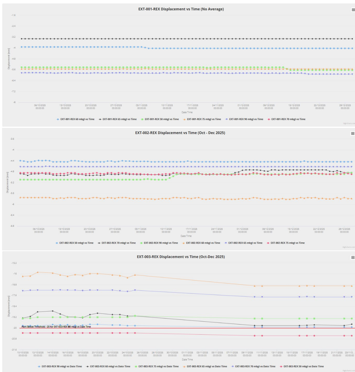
Figure 9: Displacement vs Time for REX Extensometers October – December 2025.
