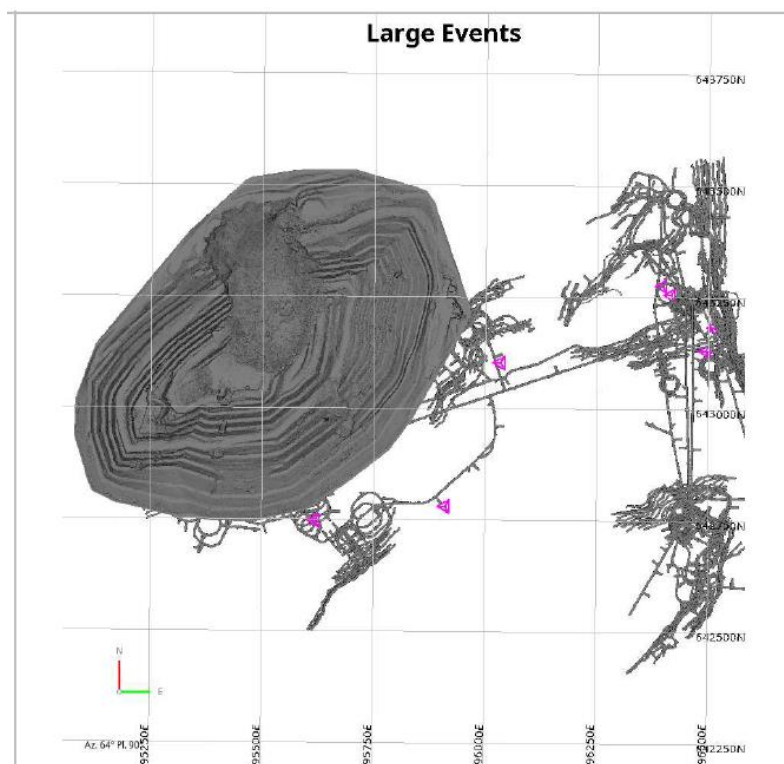
Figure 3: Plan View North highlighting locations of triggered events & reportable large events. None > ML -0.5 during January 2025.
