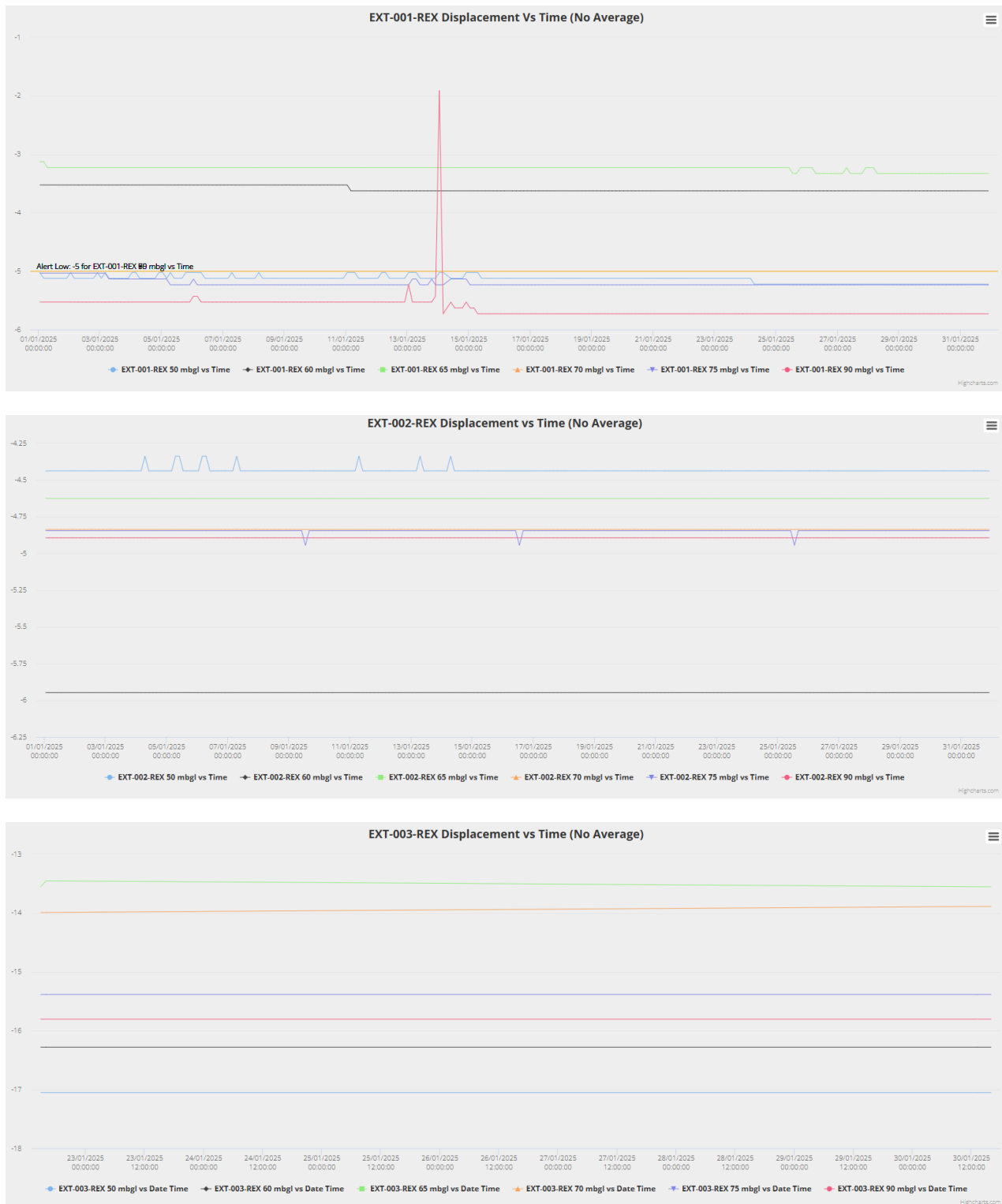
Figure 9: Displacement vs Time for REX Extensometers – January 2025.
