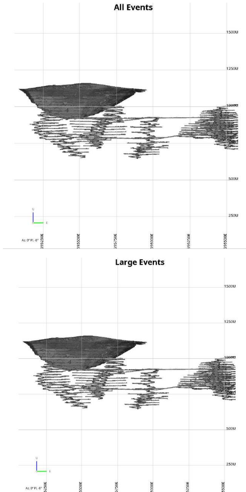
Figure 4: Section View showing location of triggered events & reportable large events. None > ML -0.5 during March 2025.
