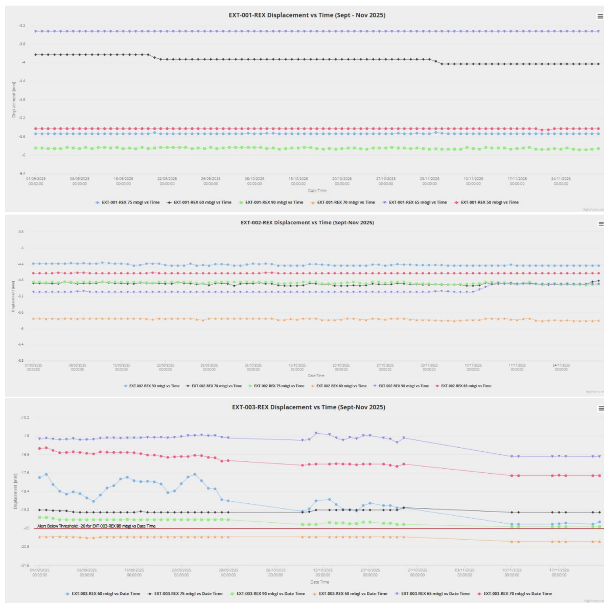
Figure 9: Displacement vs Time for REX Extensometers September – November 2025.
