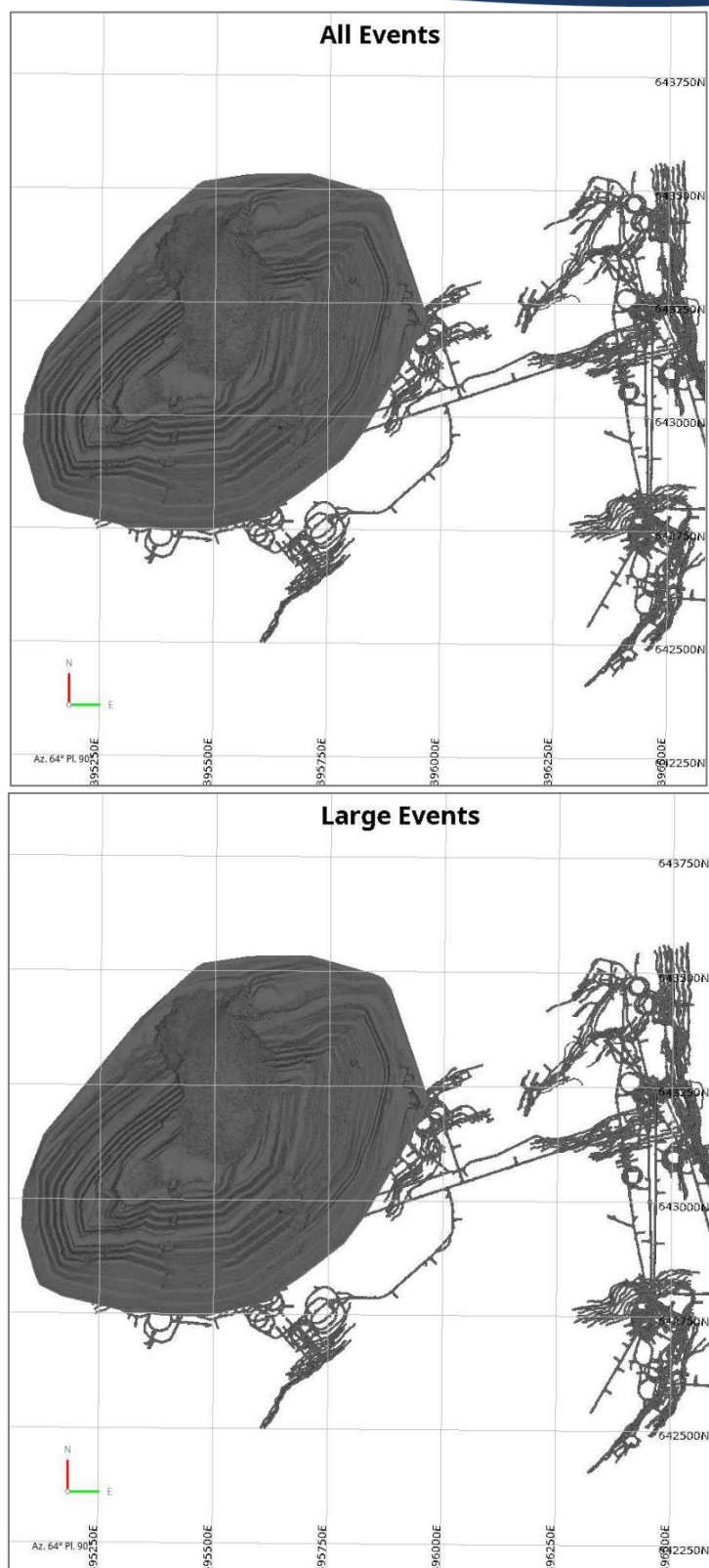
Figure 3: Plan View, Top: Normal (Location and Source) & mL \geq -3.0 & number of accepted triggers \geq 3 , Bottom: Listing of events m > -0.5 during March 2026.
