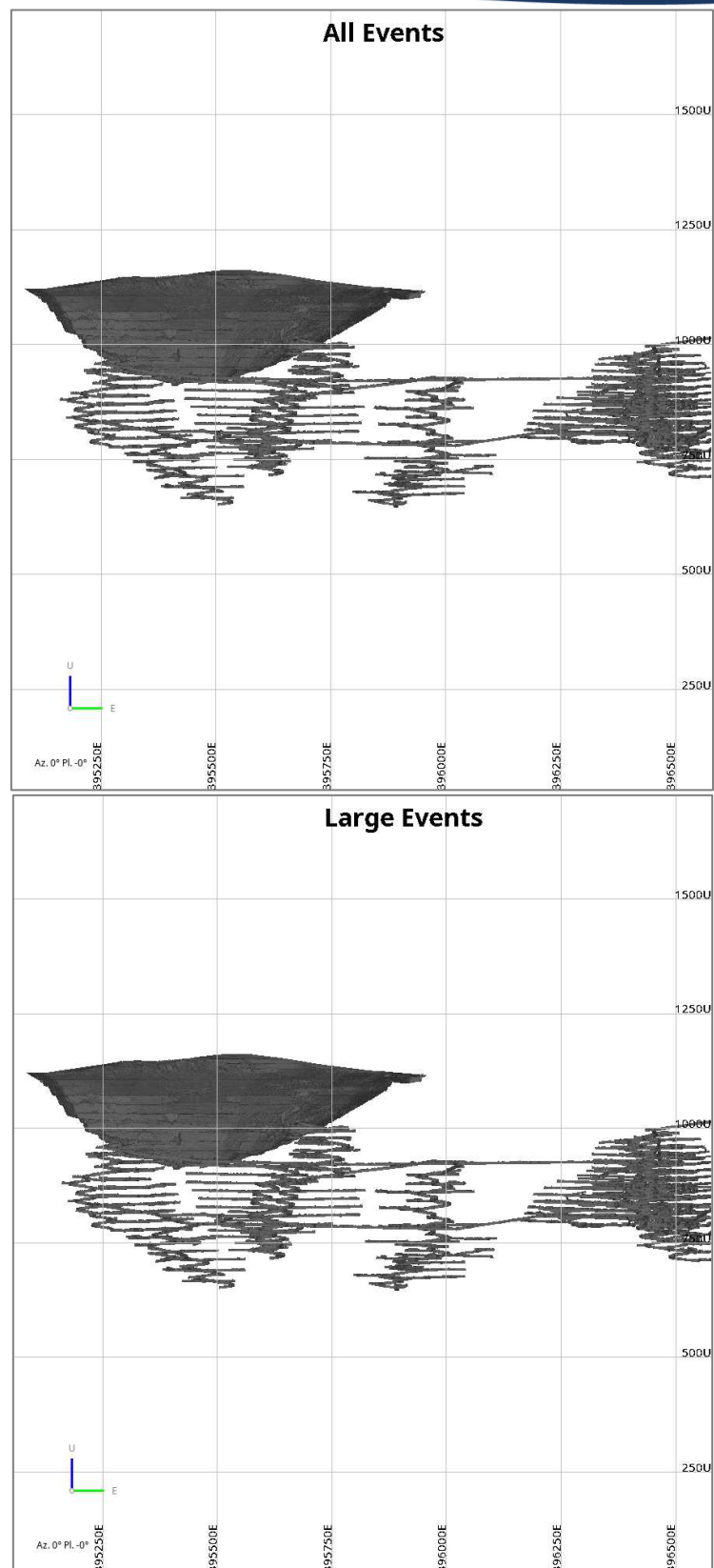
Figure 4: Looking North, Top: Normal (Location and Source) & mL \geq -3.0 & number of accepted triggers \geq 3 , Bottom: Listing of events m > -0.5 during March 2026.
