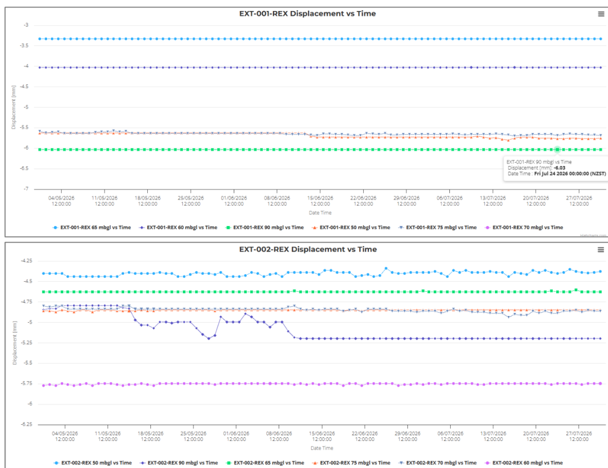
Figure 9: Displacement vs Time for REX Extensometers May - July 2026.
