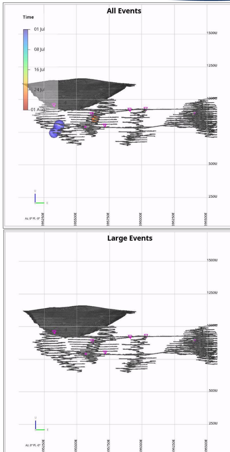
Figure 4: Looking North, Top: Normal (Location and Source) & mL \geq -3.0 & number of accepted triggers \geq 3 , Bottom: Listing of events m > -0.5 during July 2026.
