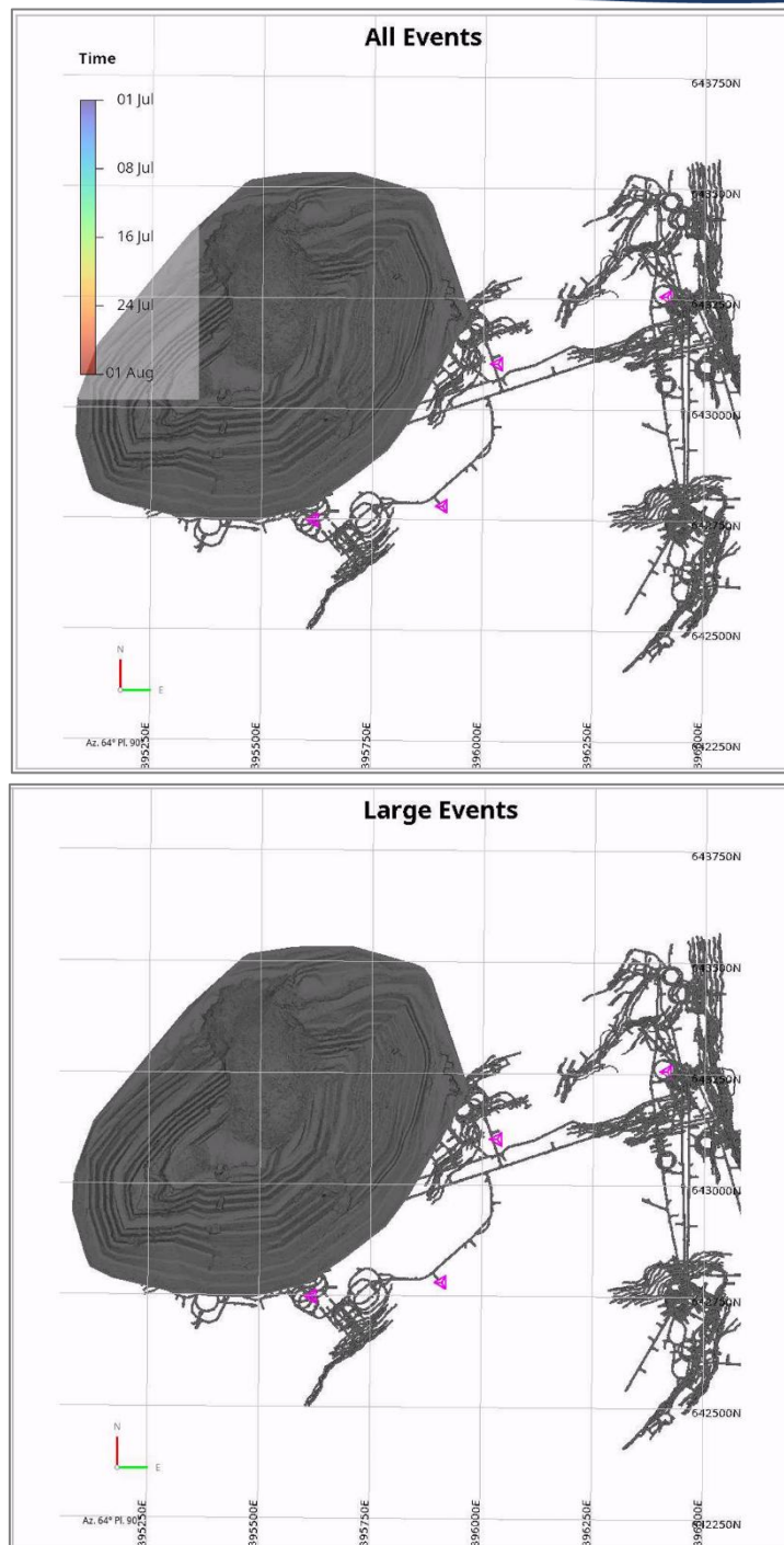
Figure 3: Plan View, Top: Normal (Location and Source) & mL \geq -3.0 & number of accepted triggers \geq 3 , Bottom: Listing of events m > -0.5 during July 2026.
