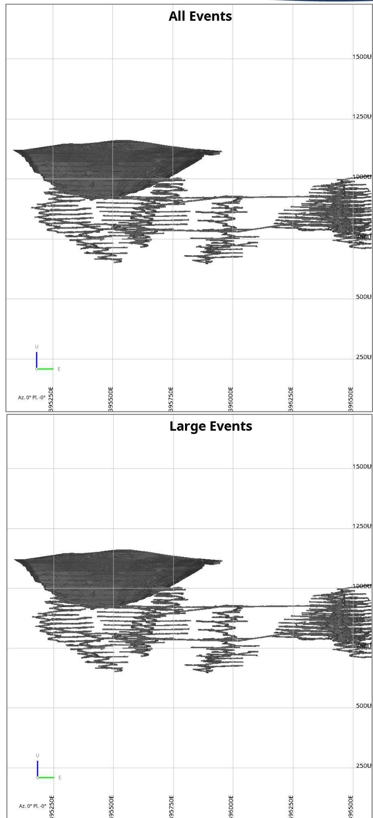
Figure 4: Looking North, Top: Normal (Location and Source) & mL \geq -3.0 & number of accepted triggers \geq 3 , Bottom: Listing of events m > -0.5 during April 2026.
