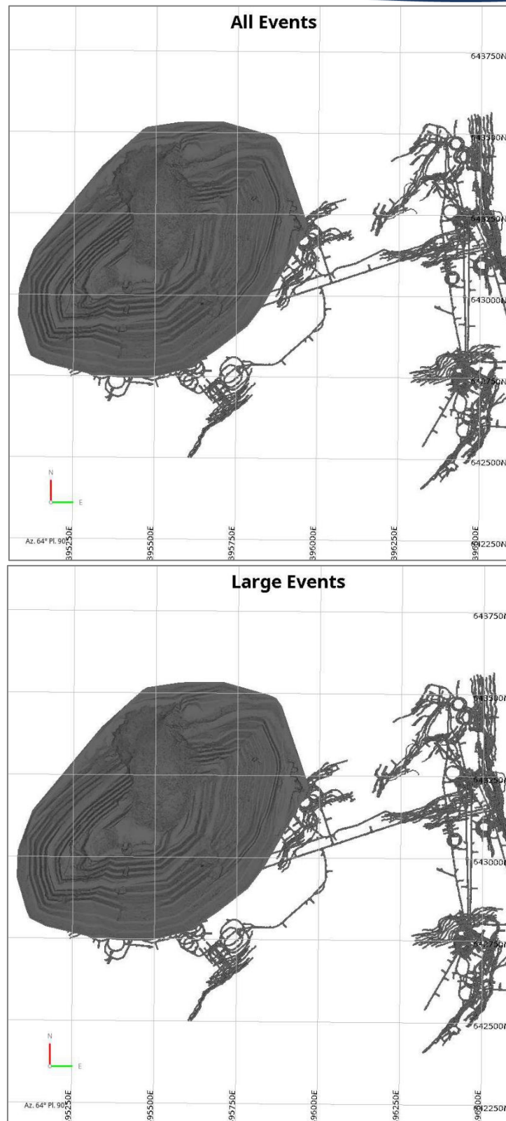
Figure 3: Plan View, Top: Normal (Location and Source) & mL \geq -3.0 & number of accepted triggers \geq 3 , Bottom: Listing of events m > -0.5 during April 2026.
