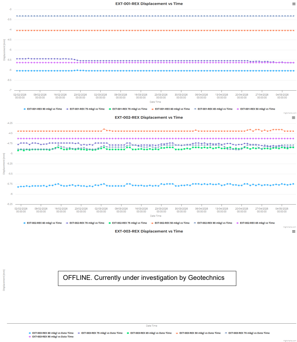
Figure 9: Displacement vs Time for REX Extensometers Feb – Apr 2026.
