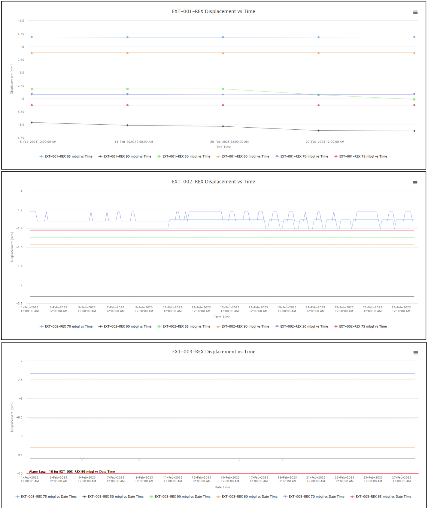
Figure 9 – Displacement vs Time for REX Extensometers – February 2023
