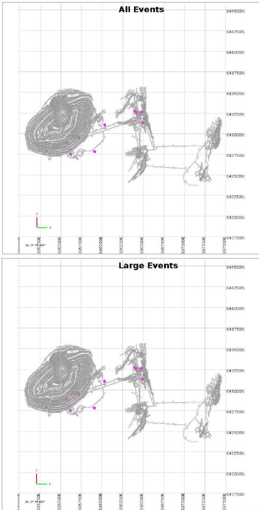
Figure 4: Plan View showing location of triggered events & reportable large events (> M-0.5 - None) during February 2023
