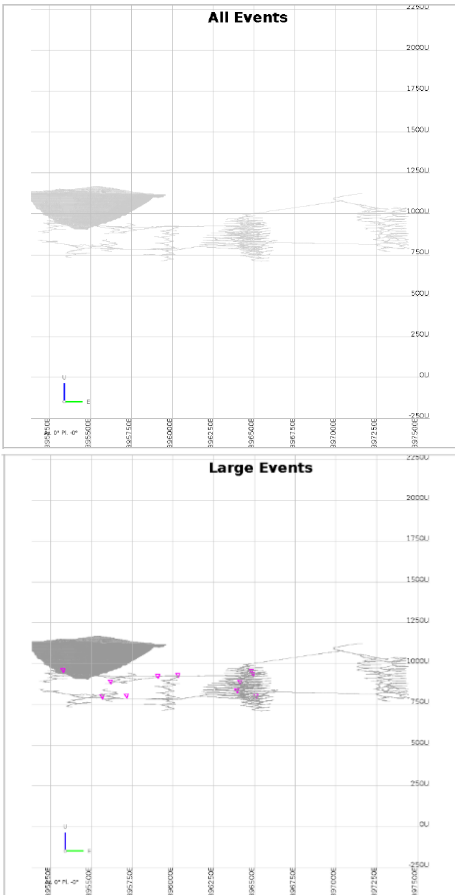
Figure 3: Section View North highlighting locations of triggered events & reportable large events. (> M-0.5 - None) during January 2024 .
