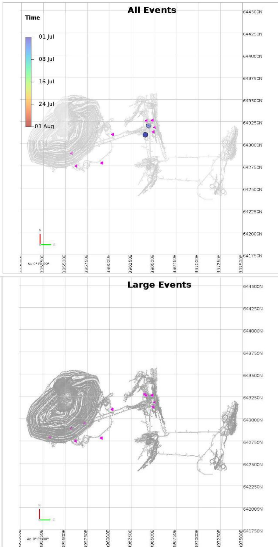
Figure 4: Plan View showing location of triggered events & reportable large events (> M-0.5 - None) during July 2023
