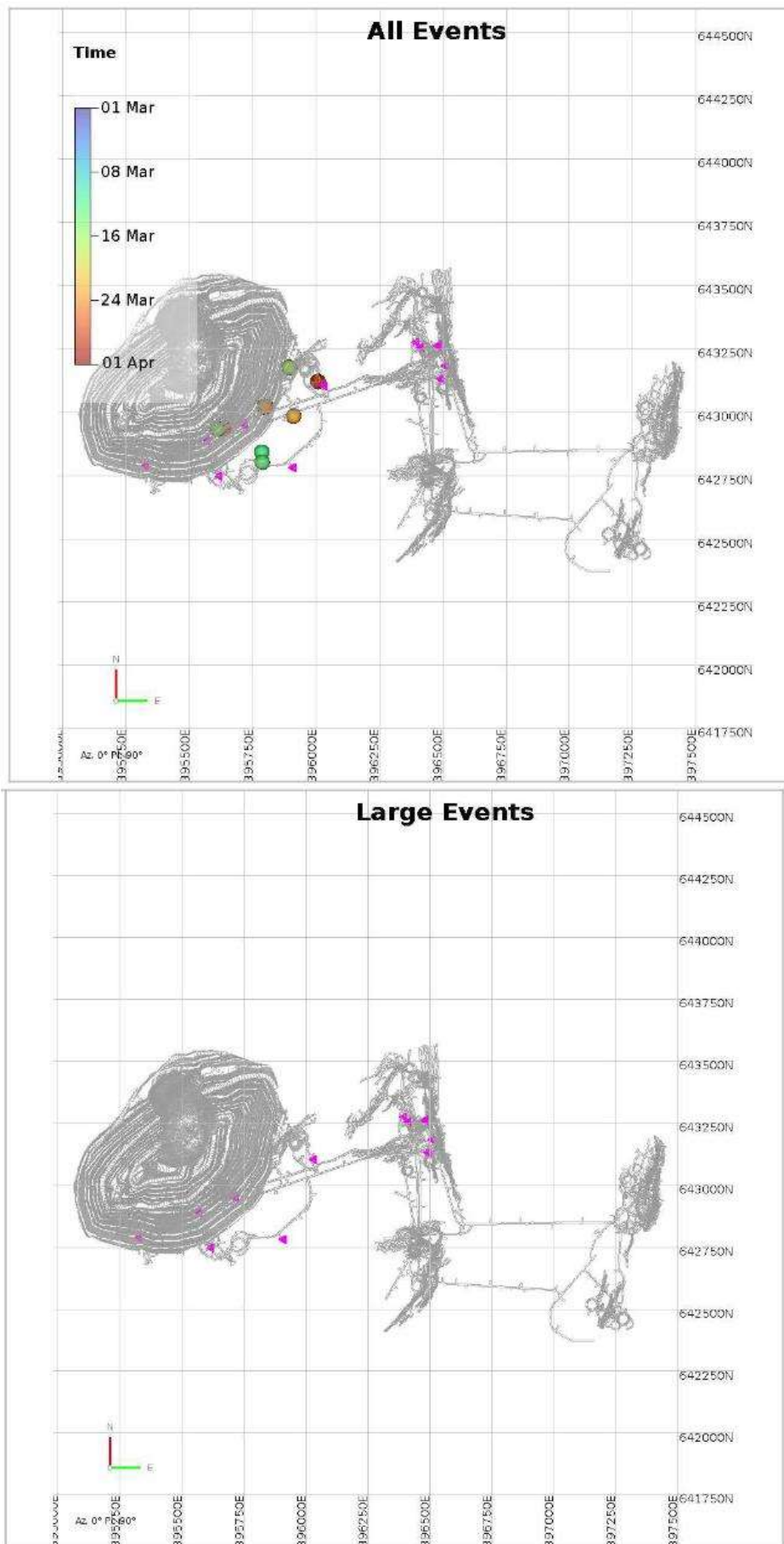
Figure 4: Plan View showing location of triggered events & reportable large events (> M-0.5 - None) during March 2023
