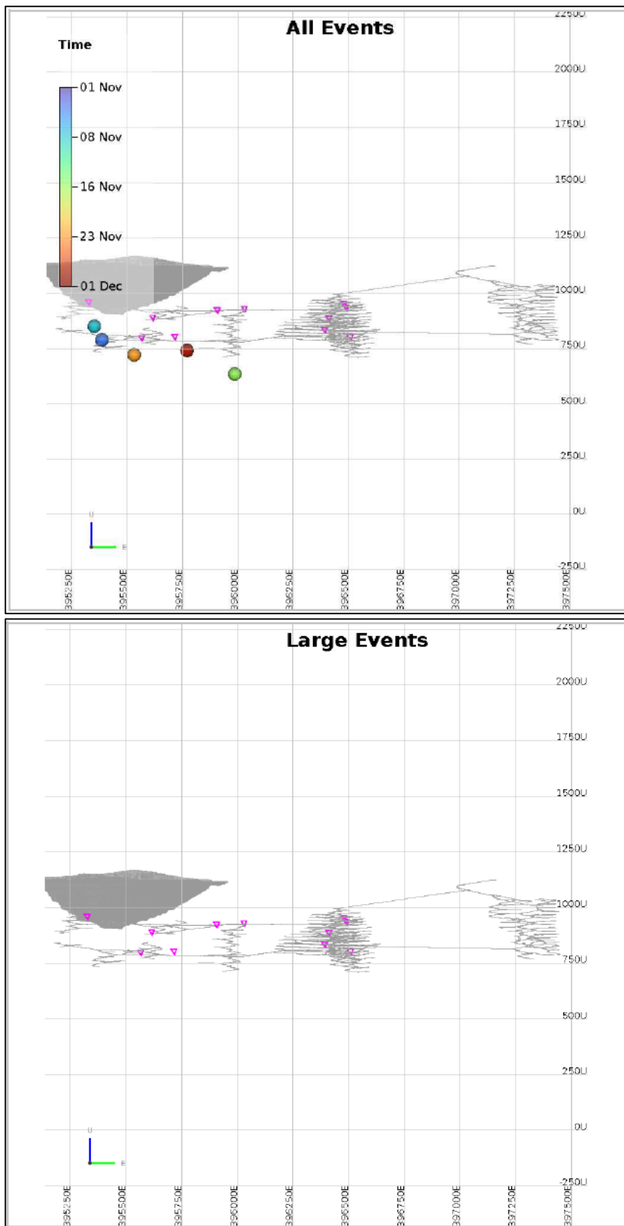
Figure 3: Section View North highlighting locations of triggered events & reportable Large events (> M-0.5 None) during November 2022
