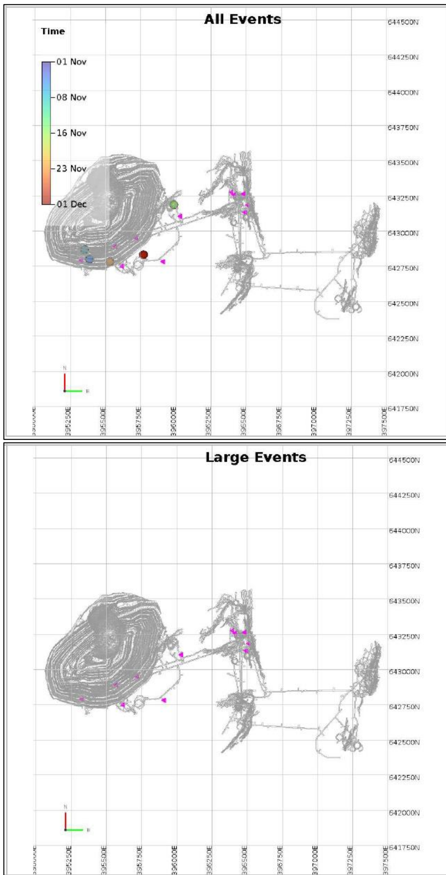
Figure 4: Plan View showing location of triggered events & reportable large events (> M-0.5 - None) during November 2022
