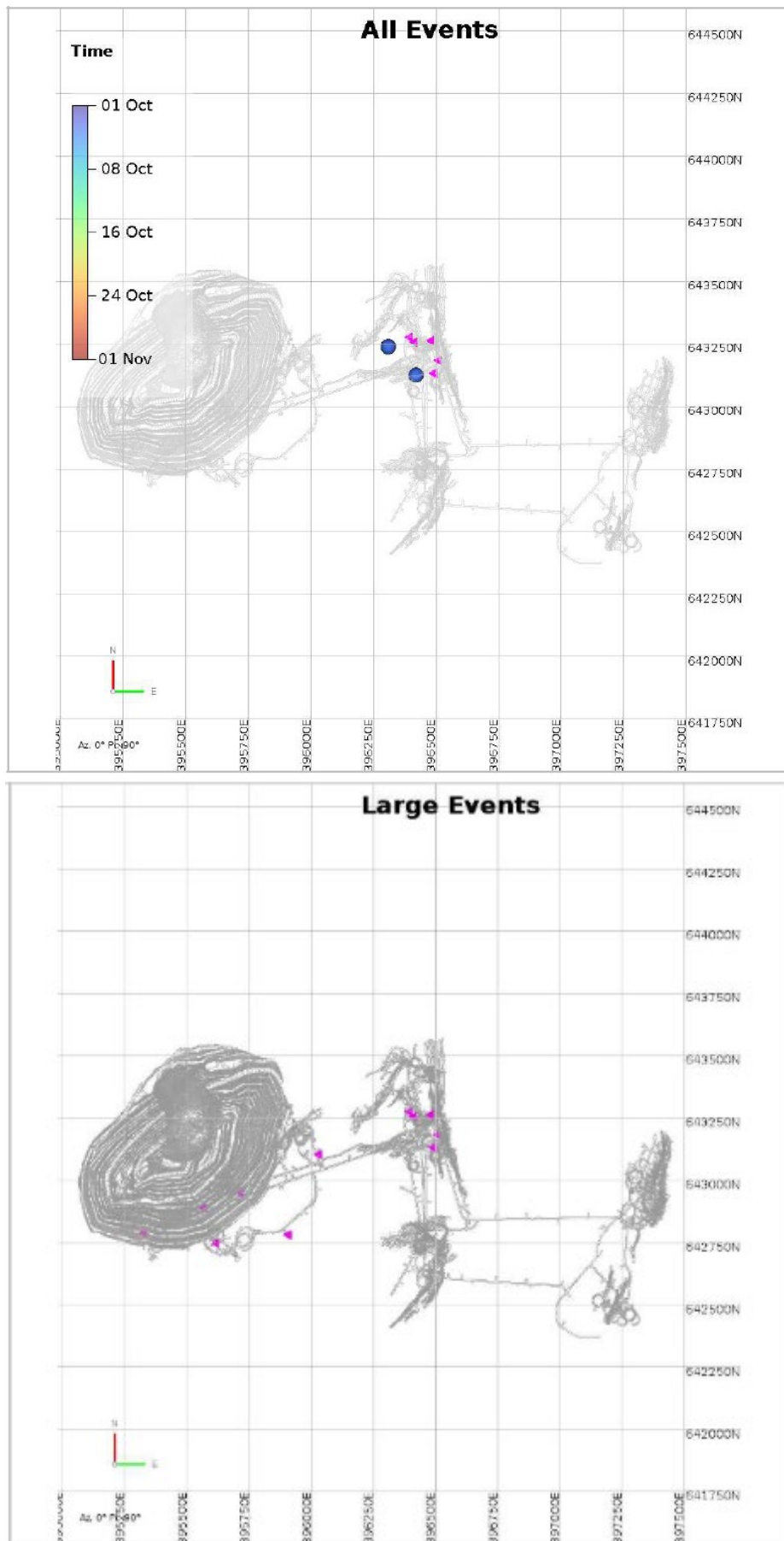
Figure 4: Plan View showing location of triggered events & reportable large events (> M-0.5 - None) during October 2023 .
