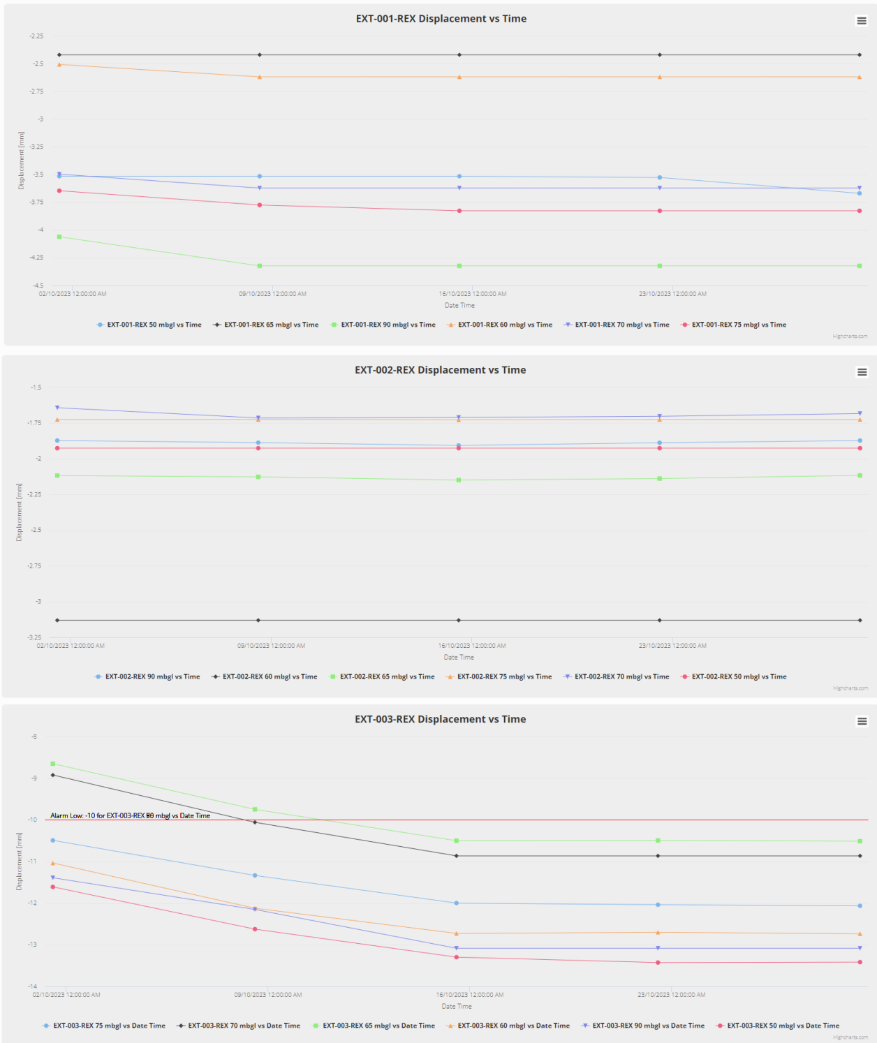
Figure 9: Displacement vs Time for REX Extensometers – October 2023.
