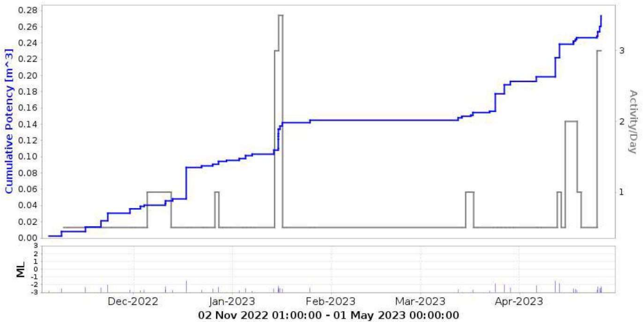
Figure 5: 180 Day Event History vs Cumulative Potency
