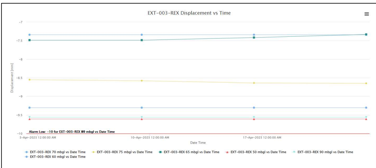
Figure 9 – Displacement vs Time for REX Extensometers – April 2023
