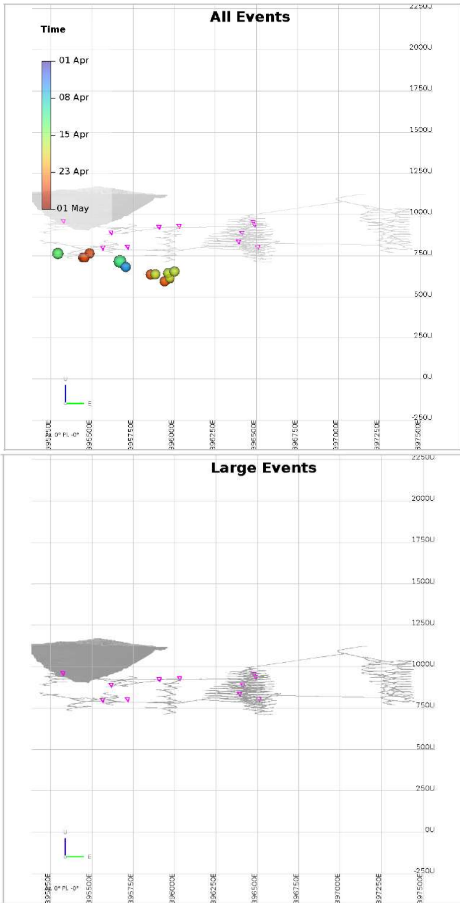
Figure 3: Section View North highlighting locations of triggered events & reportable Large events (> M-0.5 None) during April 2023
