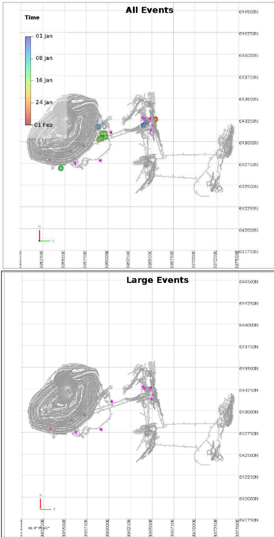
Figure 4: Plan View showing location of triggered events & reportable large events (> M-0.5 - None) during January 2023
