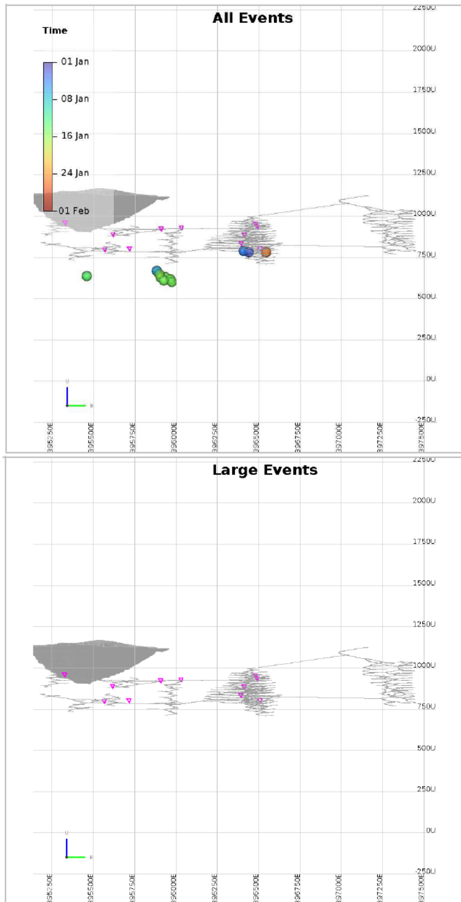
Figure 3: Section View North highlighting locations of triggered events & reportable Large events (> M-0.5 None) during January 2023
