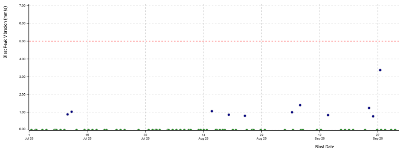
Figure 4. Maximum Peak Vibration Levels – Correnso
